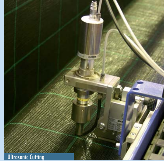
Ultrasonic Cutting
